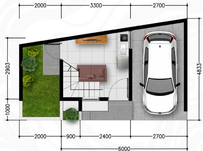
denah lantai 1
