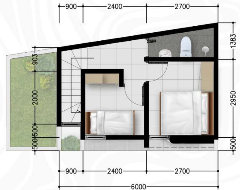
denah lantai 2
